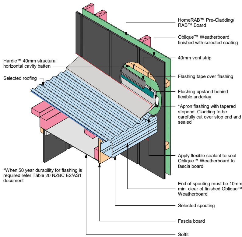
Figure 32: Roof to wall junction detail
