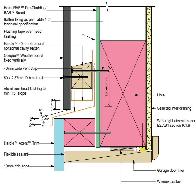
Figure 34: Garage door head
