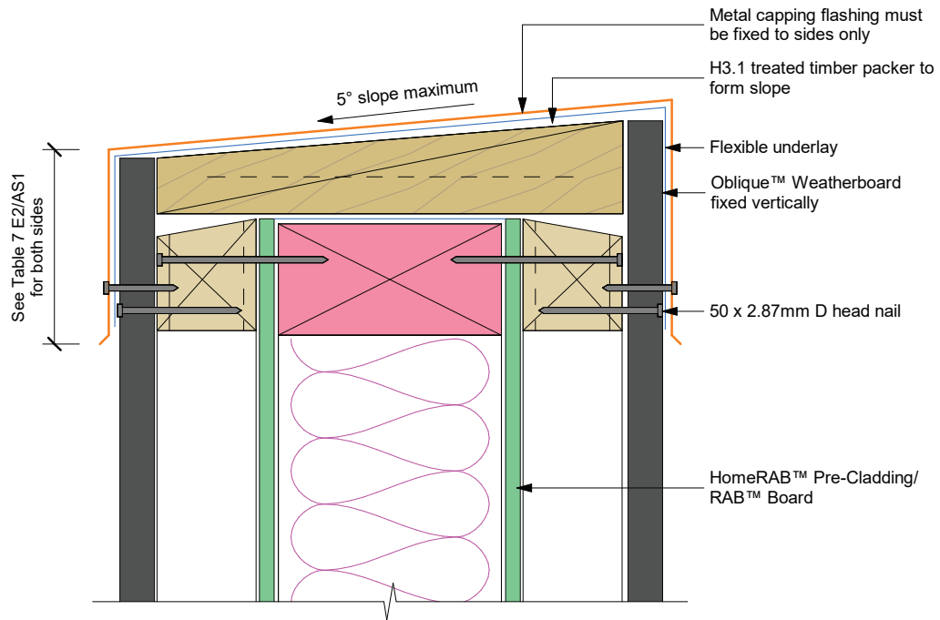
Figure 32: Roof to wall junction detail
