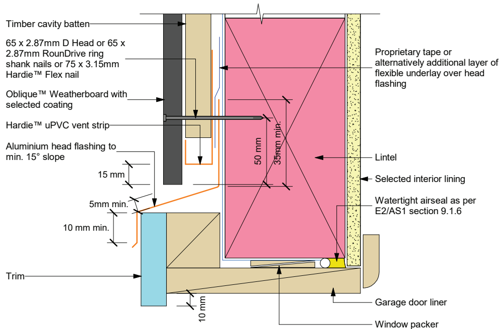
Figure 41: Garage head
