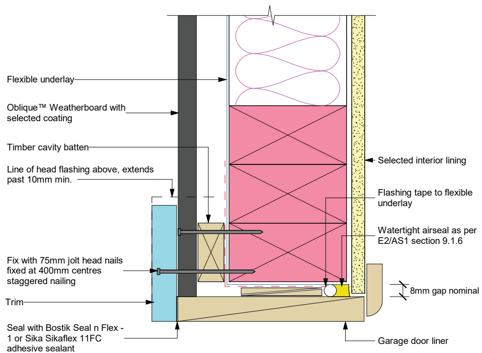
Figure 42: Garage jamb
