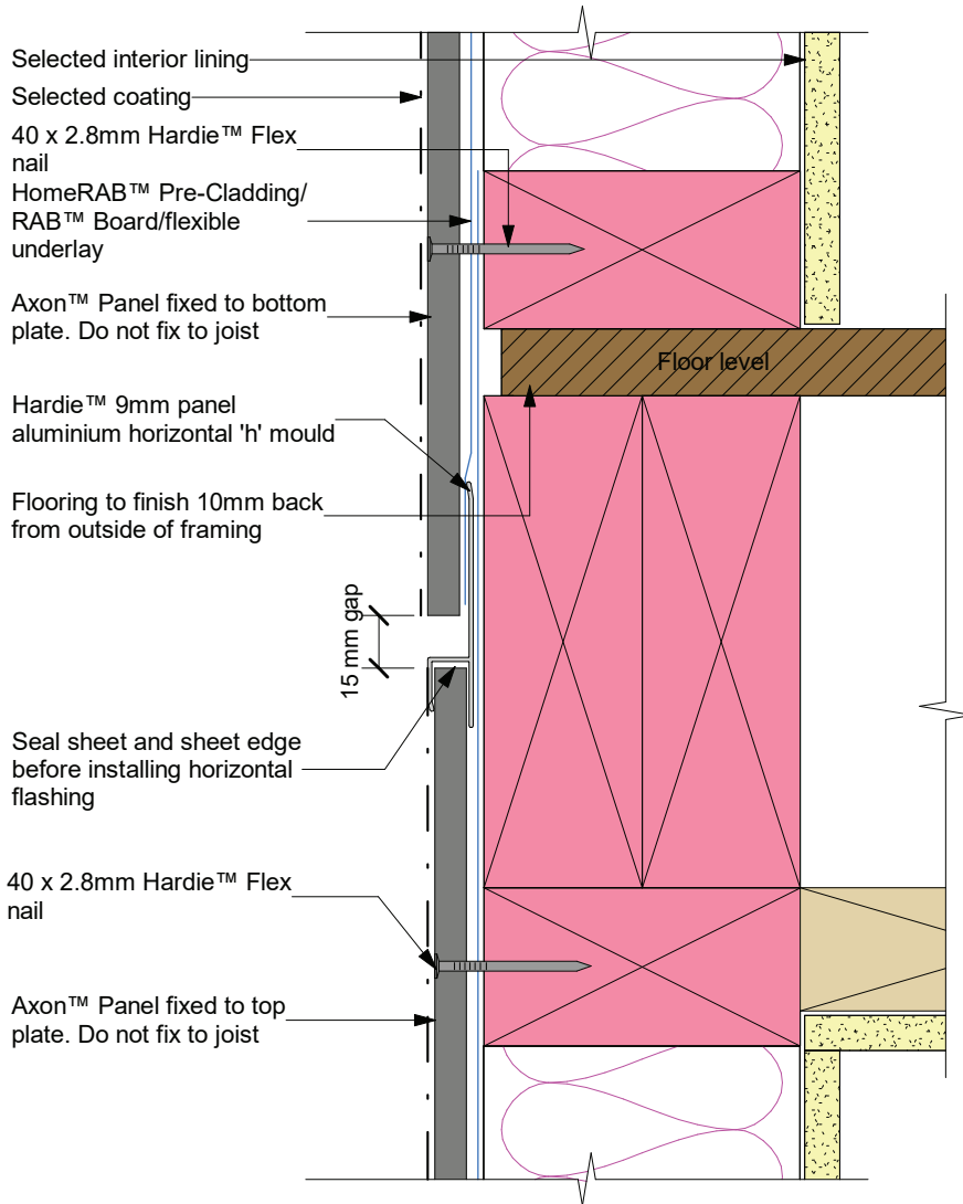
Figure 20: Horizontal joint detail
